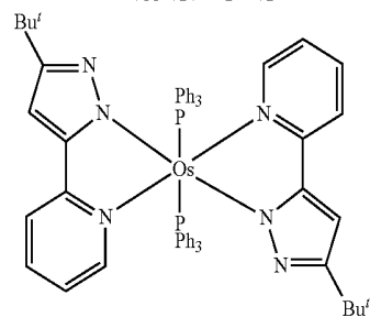
Os(bppz) 2 (PPh 3 ) 2
