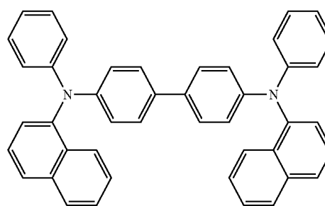
NPB
